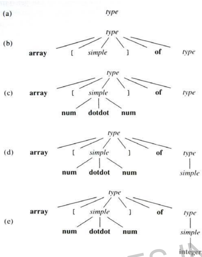
Fig 2.11. Steps in the top-down construction of a parse tree.
