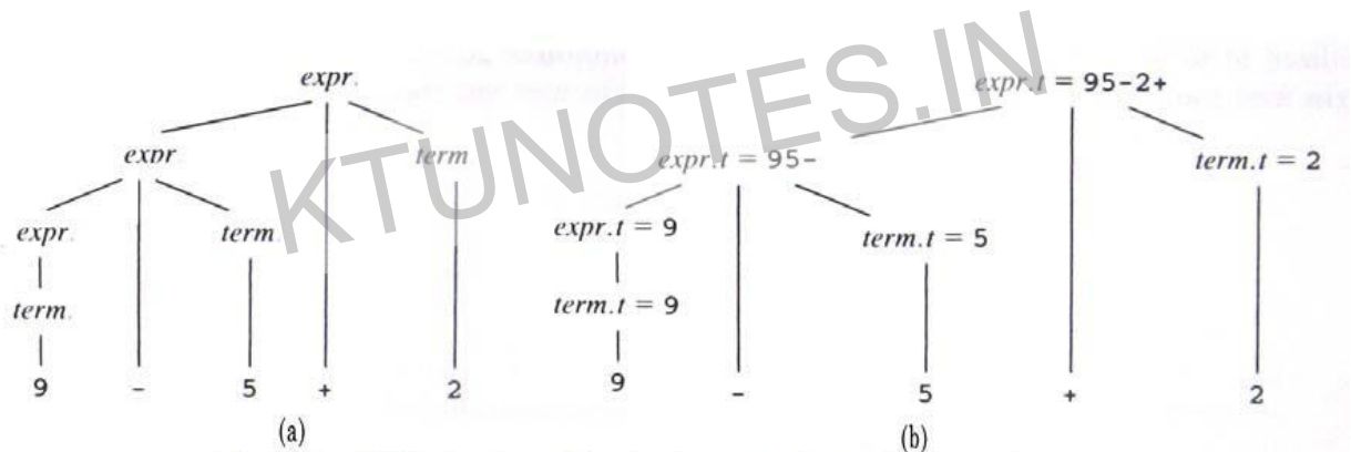
Fig 2.6. Attribute values at nodes in a parse tree.
