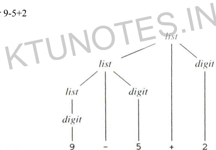
Fig 2.2. Parse tree for 9-5+2 according to the grammar in Example
